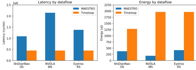
Figure 1: Latency (cycles) and energy ( \mu J) by dataflow for MAESTRO and Timeloop on the same 107M-MAC layer (256-PE equivalent).
