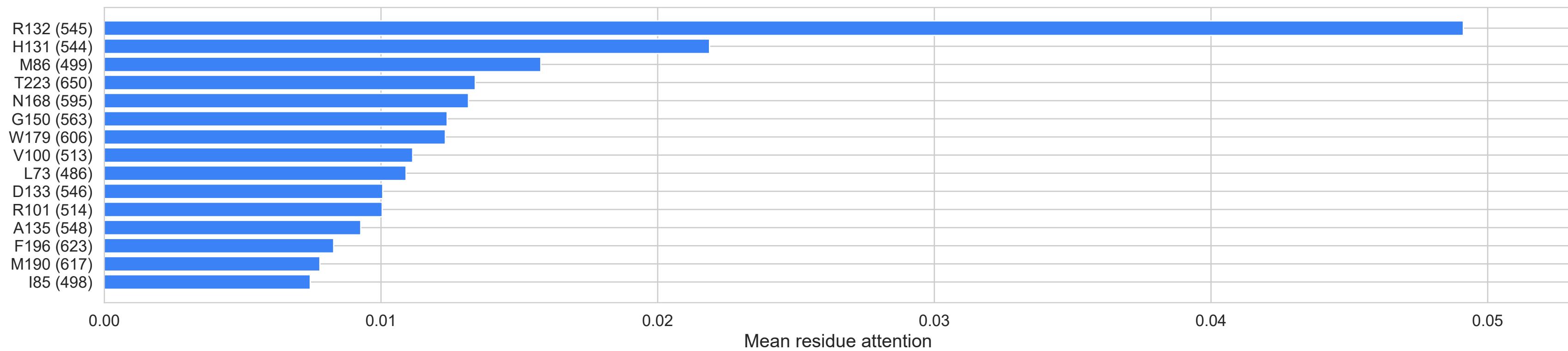
Residue attention versus structure-derived contacts
