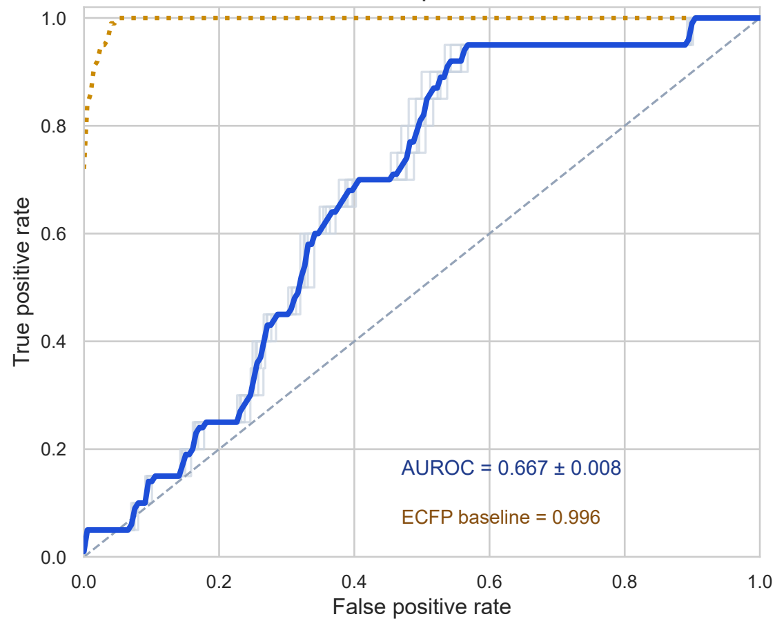
ROC across replicate libraries
