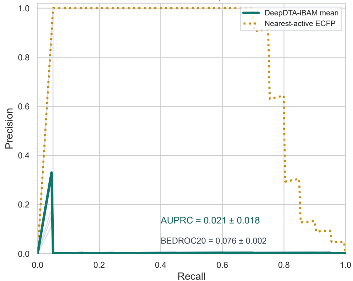
Precision-recall across replicate libraries
