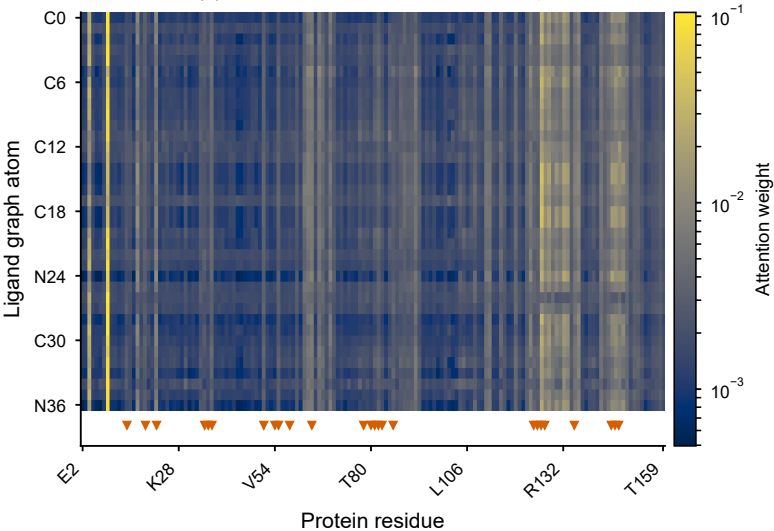
(a) ABL1 + imatinib: the interaction map
