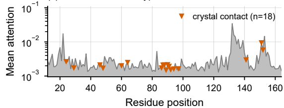
(c) EGFR + erlotinib, type I: AUROC 0.424, at chance
