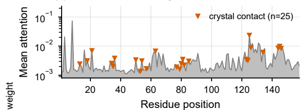
(b) Same complex, averaged over atoms: AUROC 0.709
