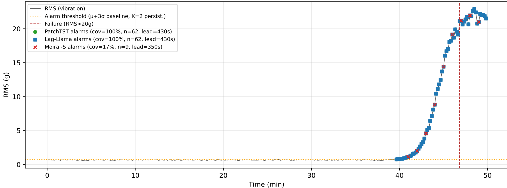
Missed-alarm cascade — Bearing1_1 (action window: 300s)
