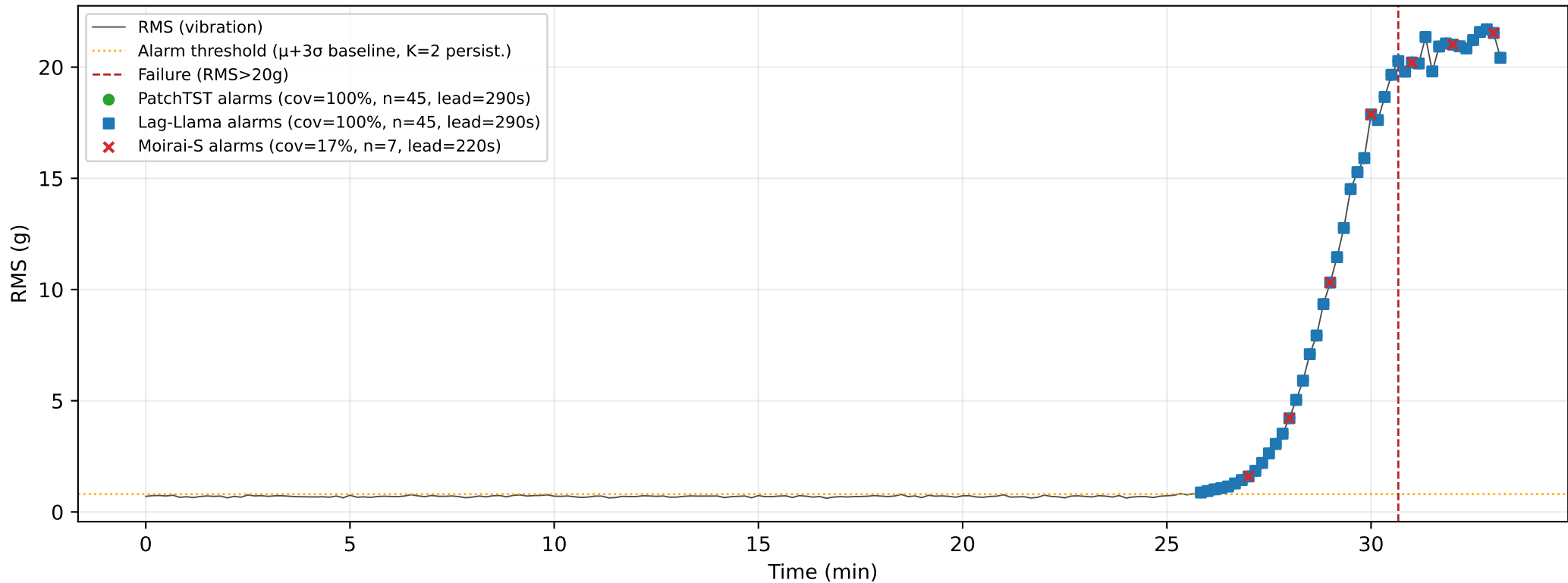
Missed-alarm cascade — Bearing1_2 (action window: 300s)
