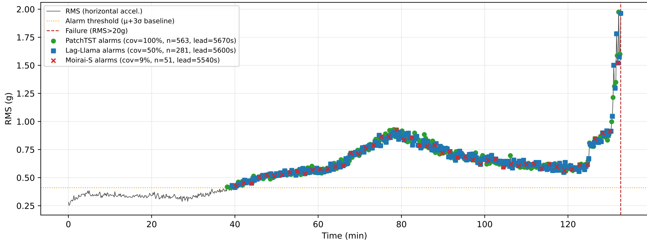
Missed-alarm cascade — Bearing2_2 (action window: 300s)
