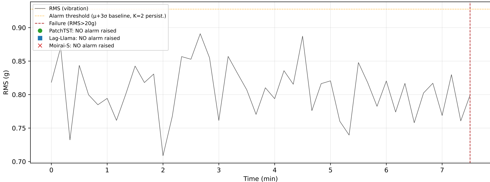
Missed-alarm cascade — Bearing2_1 (action window: 300s)
