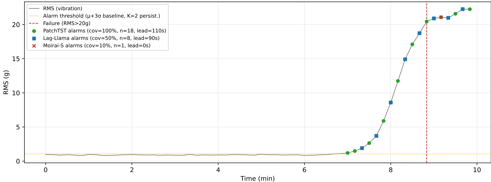
Missed-alarm cascade — Bearing3_2 (action window: 300s)
