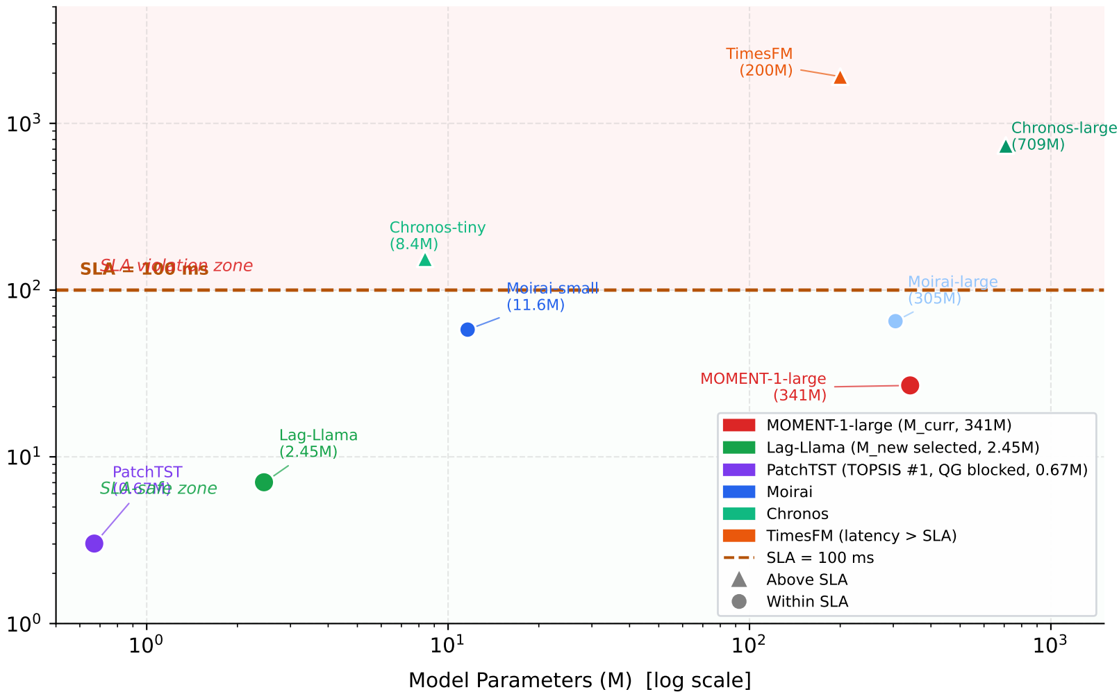
Mean Inference Latency (ms) [log scale]
