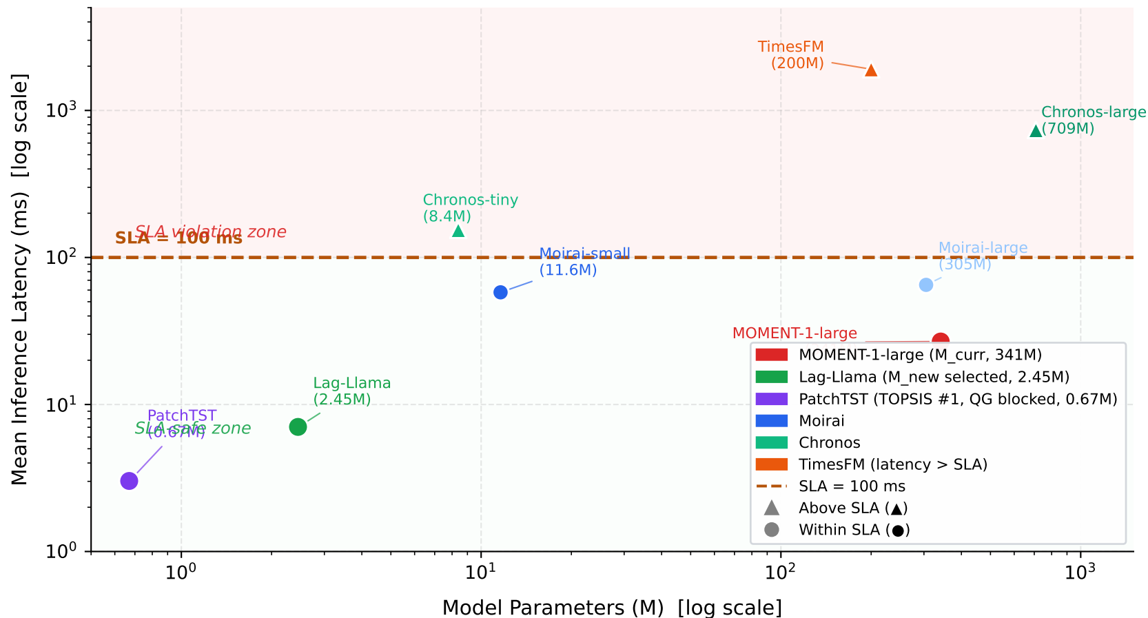
Fig. 1 — Benchmark: Inference Latency vs. Model Size on ETT-h1 (GPU T4, 2026-04-07) MOMENT-1-large = M_curr | Lag-Llama = M_new selected | PatchTST = TOPSIS #1 (QG blocked)
