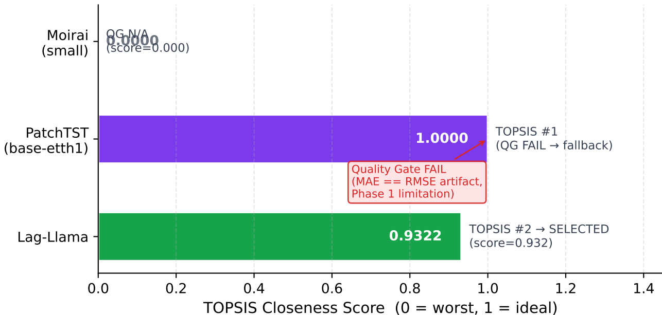
Fig. 2 — Stage 2: TOPSIS Ranking of Candidate Models Weights: w_{MAE}=0.5 , w_{lat}=0.3 , w_{params}=0.1 , w_{lic}=0.1
