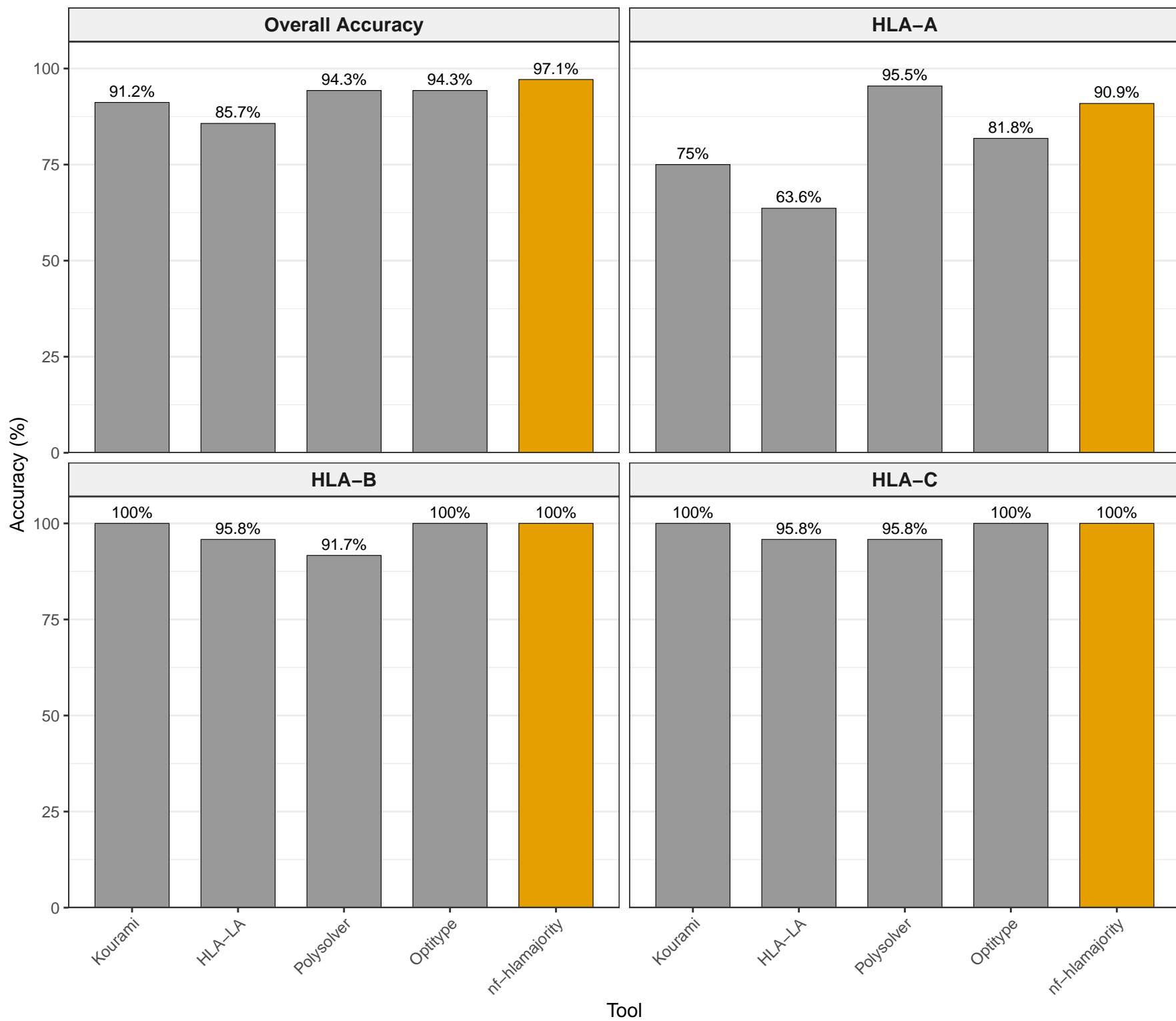
Genotyping Accuracy by Tool and Gene Comparison with NCI-60 WES Dataset
