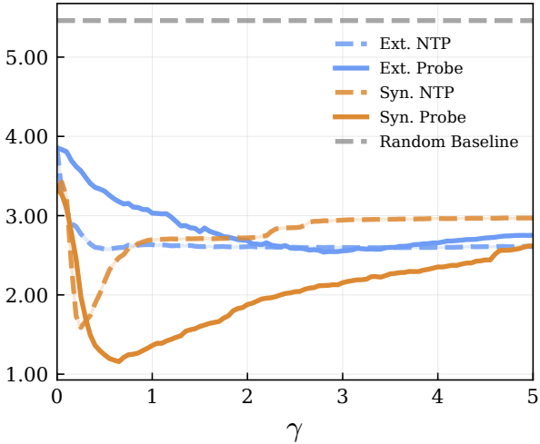
Mean Centroid Distance
