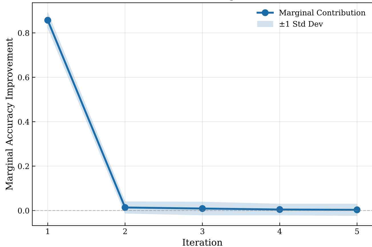
Iterative Head Selection: Marginal Contributions
