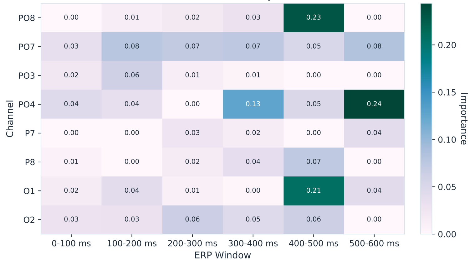
SVM Channel x Time Importance
