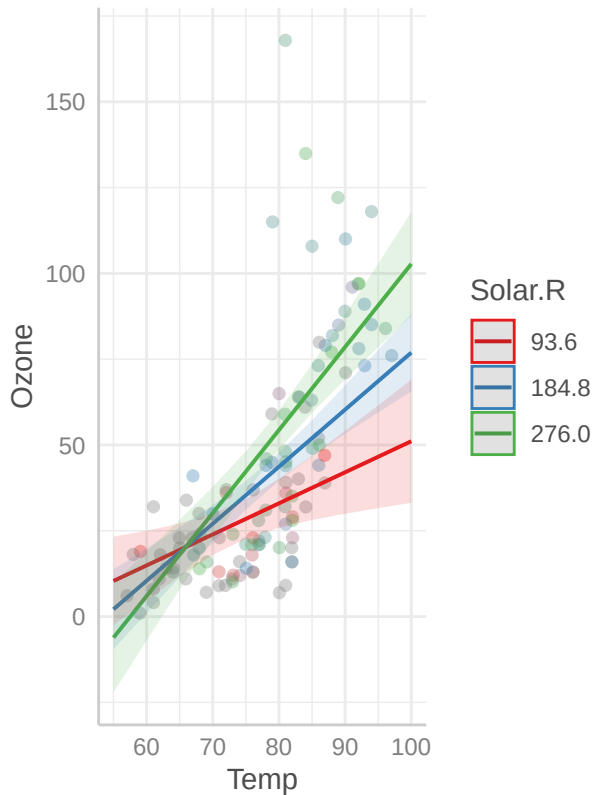
Predicted values of Ozone
