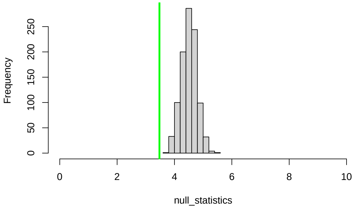
Histogram of null_statistics
