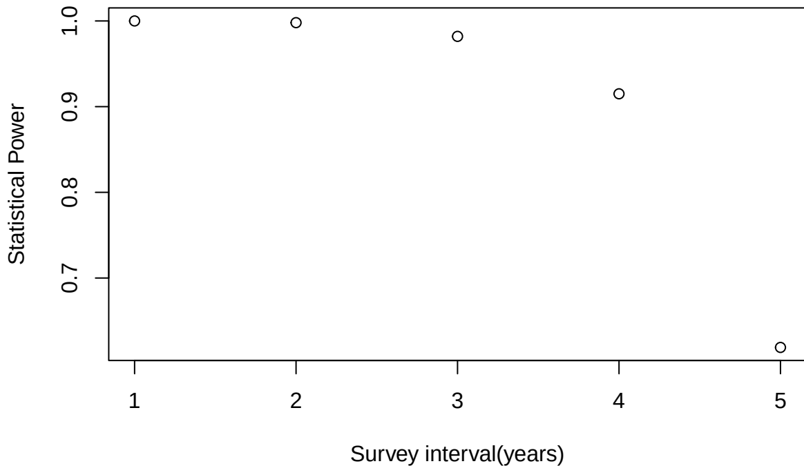
Power to detect trend, by sampling interval
