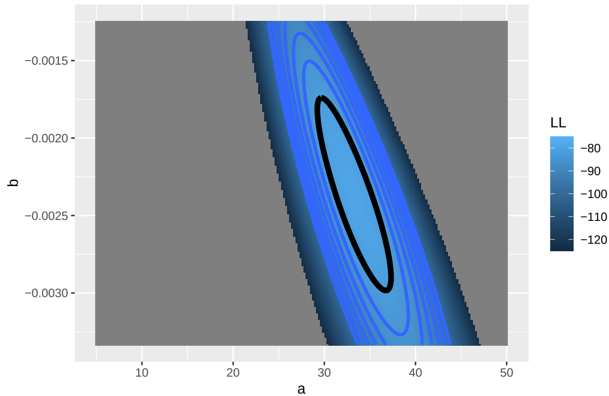
Log Likelihood Surface with 2D Confidence Region
