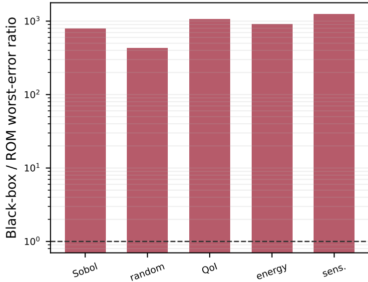
(b) Ratio at 20 materials
