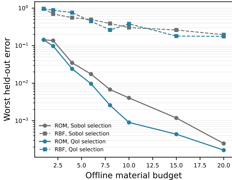
(a) Structure-aware vs black-box
