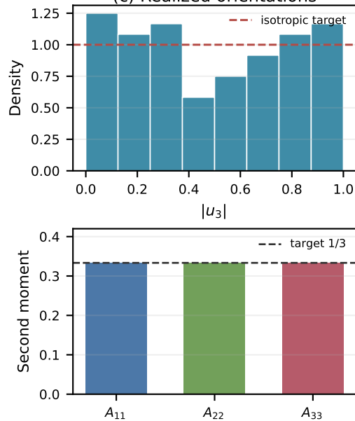
(c) Realized orientations
