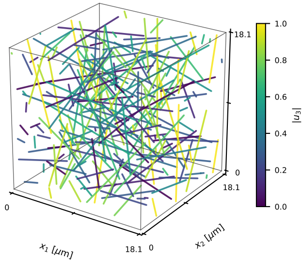
(a) Continuous periodic fibers ( n_f = 96 )
