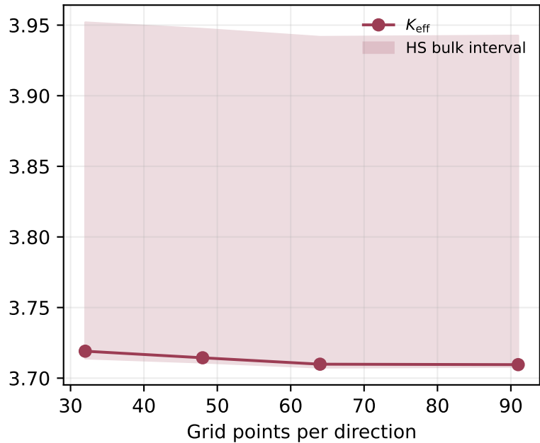
Bulk modulus
