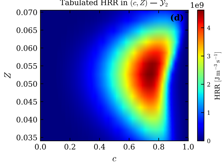
Tabulated HRR in (c, Z) — \mathcal{Y}_2
