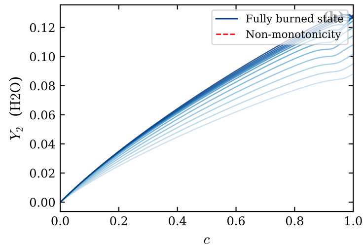
Flamelet profiles — Y_2 (H 2 O)
