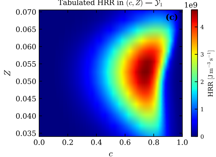
Tabulated HRR in (c, Z) — \mathcal{Y}_1
