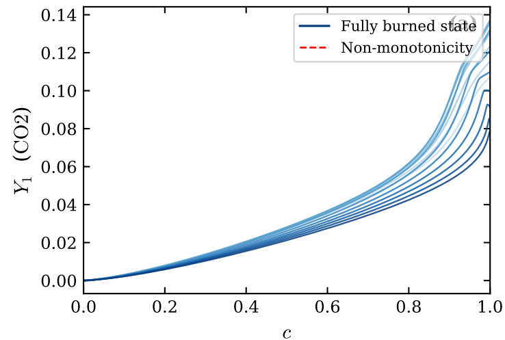
Flamelet profiles — Y_1 (CO 2 )
