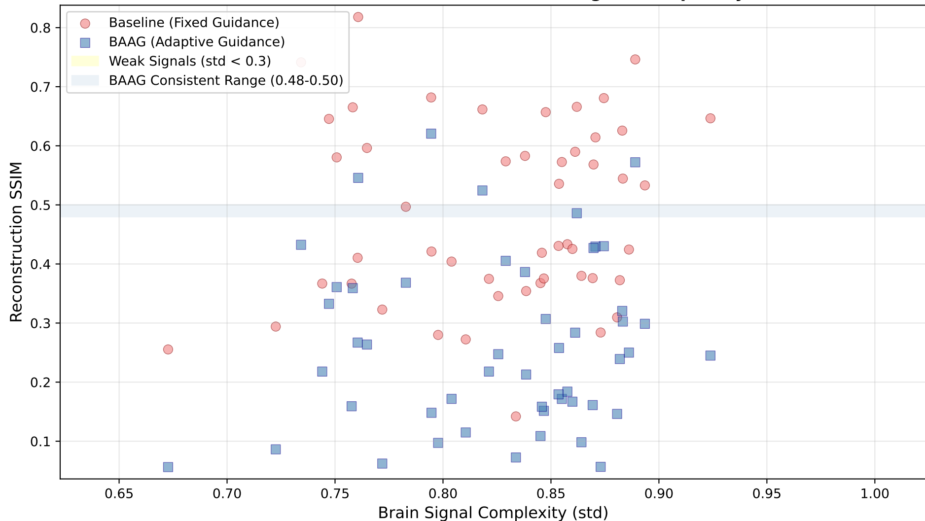
Reconstruction SSIM versus Brain Signal Complexity
