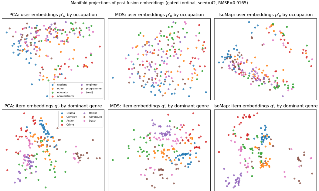
Figure 4: Two-dimensional projections of the post-fusion user representations p'_u (top, coloured by occupation) and item representations q'_i (bottom, coloured by dominant genre). Columns show PCA, classical MDS, and IsoMap with k = 15 neighbours. Item-side genre structure is recovered most clearly by IsoMap; user-side occupation structure is present in the high-dimensional space but does not survive projection to two dimensions.
