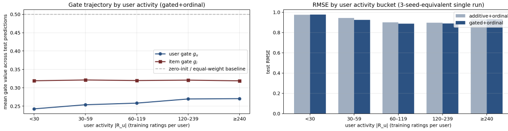
Figure 3: Per-bucket cold-start analysis. Left: mean per-prediction gate value across user-activity buckets. Both gates settle around g_u \approx 0.25 and g_i \approx 0.32 , well below the zero-initialisation value of 0.5, and are nearly flat across activity. Right: test RMSE by user-activity bucket for the two fusion variants. Gated fusion’s advantage concentrates in the mid-activity range; cold and power users see no benefit.
