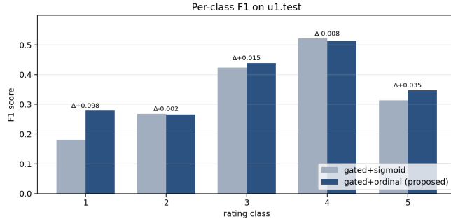
Figure 1: Per-class F1 on u1.test . The ordinal head mainly improves the boundary classes, rather than creating a uniform gain across all ratings.
