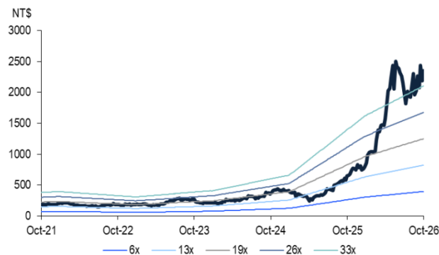
Figure 3. Chroma ATE – 12M Fwd. P/E Band
