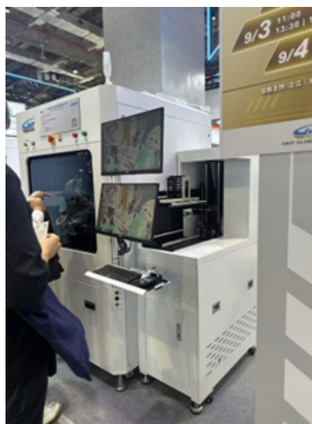
Exhibit 2: GMT FAU active alignment and bonding system
