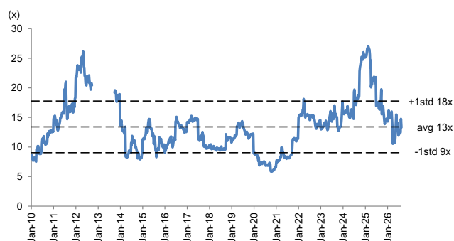
Exhibit 5: Compal's 12M forward P/E
