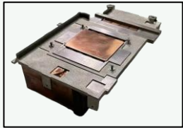
Thermal Solution for AI desktop D8 Heat pipe Solution CPU+GPU 55~85Watts
