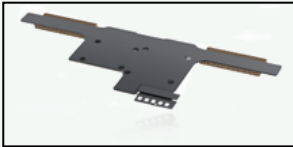
Thermal Solution for Gaming Laptop Slim VC ( 1.4\text{mm} \leq t \leq 2.5\text{mm} ) CPU+GPU 90~220 Watts
