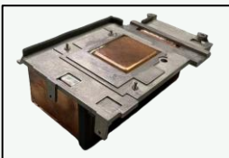
Thermal Solution for AI desktop vapor chamber Solution CPU+GPU 95~120Watts
