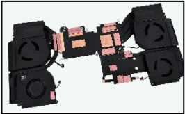
Thermal Solution for Gaming Laptop VC( 1.2\text{mm} \leq t \leq 3.5\text{mm} ) increases volume for CPU+GPU 90~320 Watts
