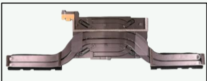
Thermal Solution for AI Laptop D6+D8 Heat pipe Solution CPU 110Watts
