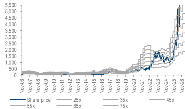
GUC: 4-quarter forward PER bands
