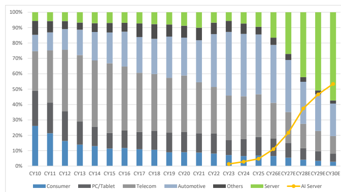
Figure 5: MLCC industry sales breakdown forecast by application
