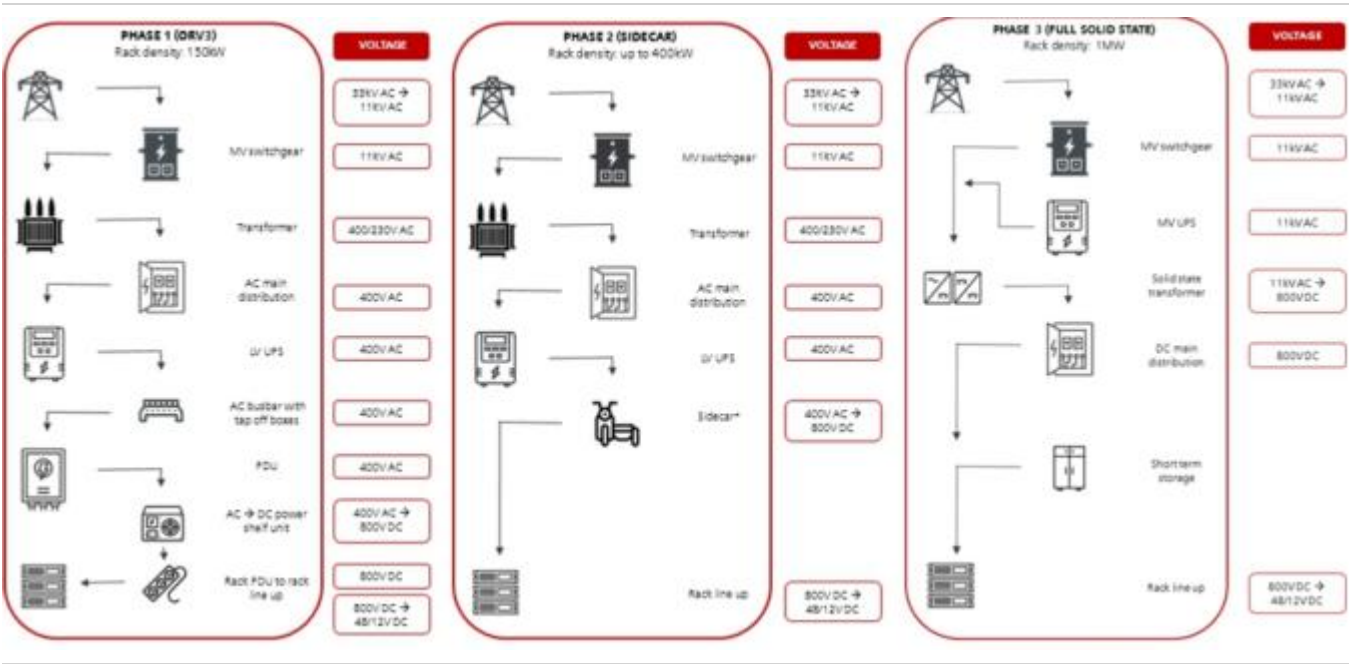
Figure 11: Three phases of 800V DC architecture
