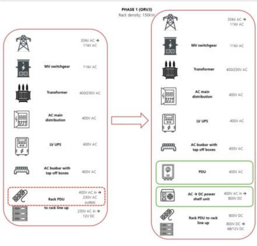
Figure 15: Evolution of current architecture to Phase 1
