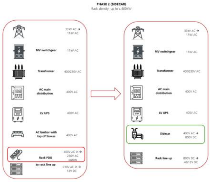
Figure 17: Evolution of current architecture to sidecar
