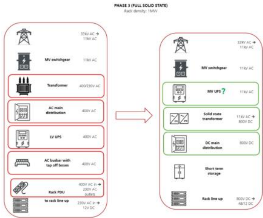
Figure 19: Evolution of current architecture to full solid state
