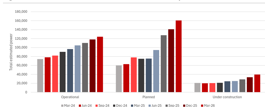
Figure 21: UBS Evidence Lab - Global Data Centre Exposure Monitor
