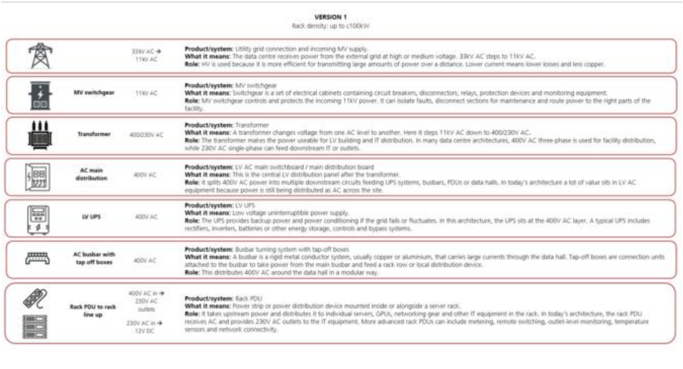
Figure 12: Current data centre architecture (version 1)
