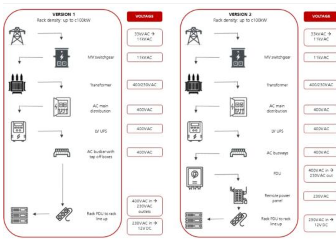
Figure 10: Data Centre architecture available today
