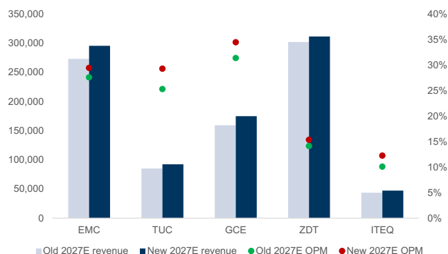
Exhibit 2: We expect revenue and OPM in 2027E to see more upside driven by price hike NT$m
