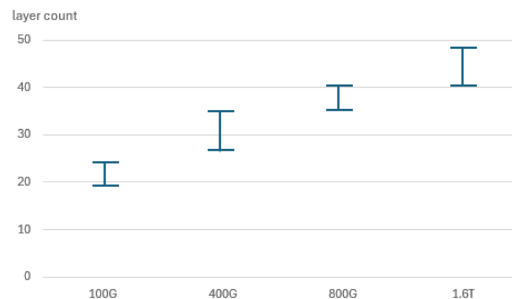
PCB layer count comparison (switch as illustration)
