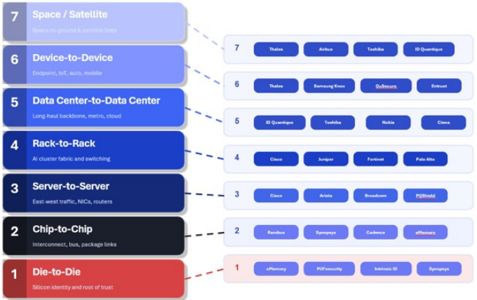
Exhibit 4: Quantum security across different connectivity layers
