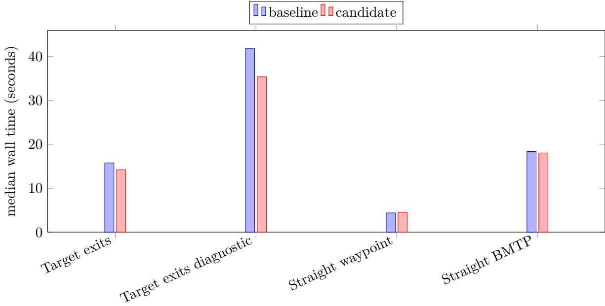
Figure 6: Measured median wall times from verification.md . Each pair compares the recorded baseline and candidate medians for one timed case.
