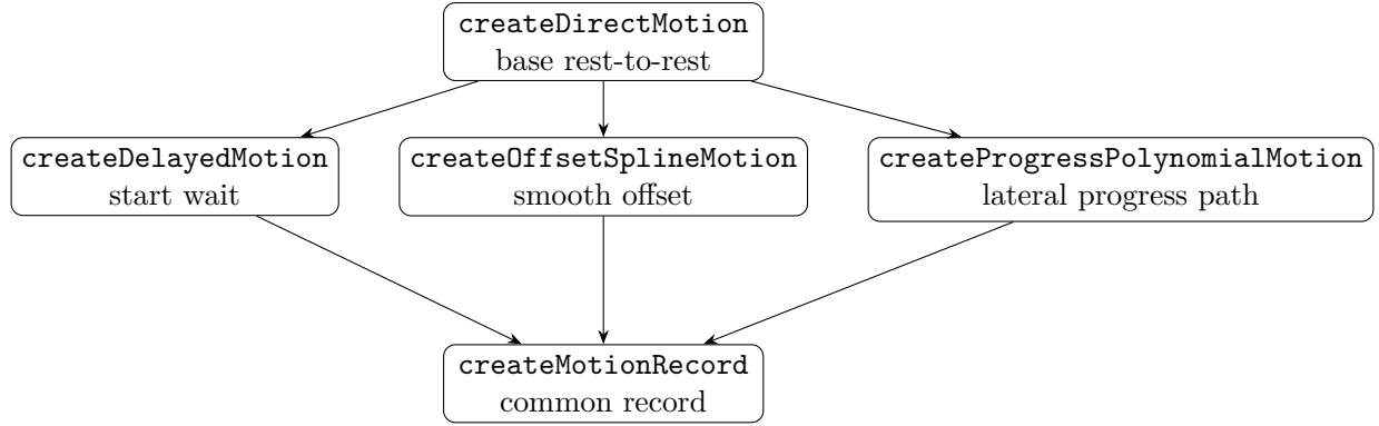
Figure 5: How exact motion builders create a common candidate record.
