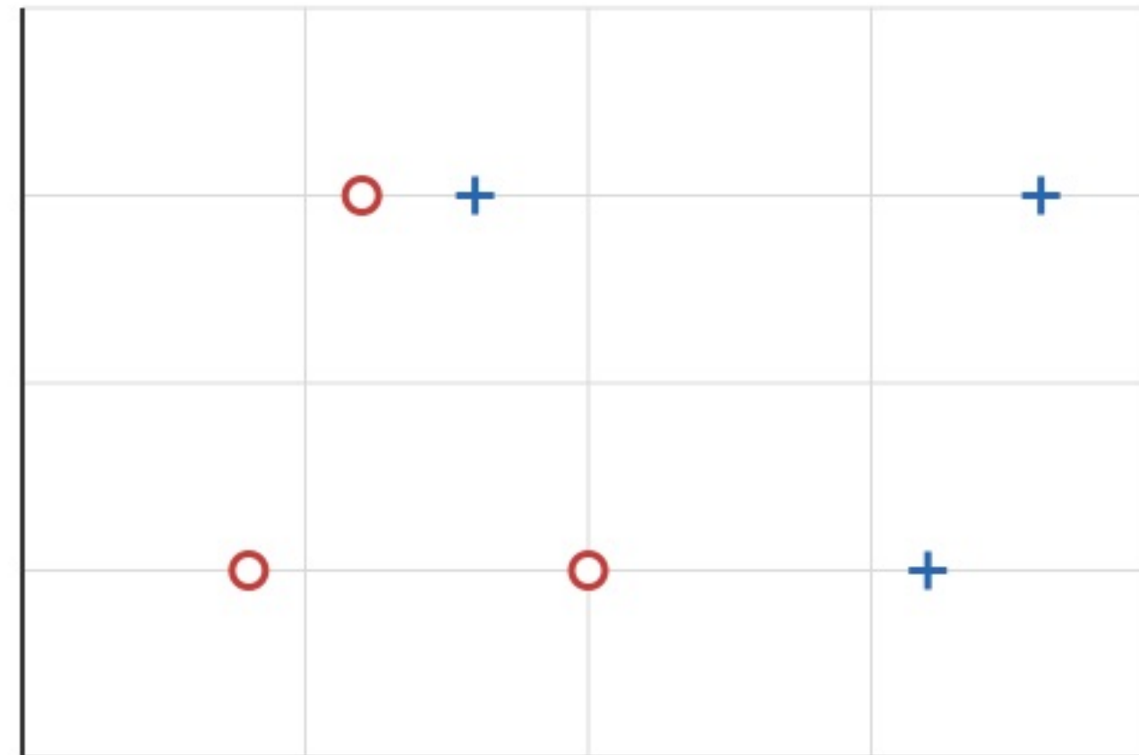
(c) V_1 vs. V_3
