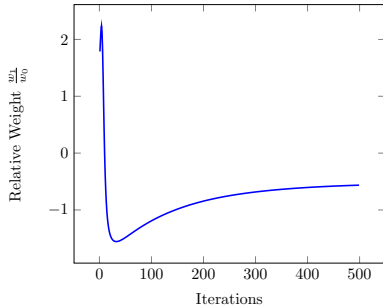
(b) Weight \frac{w_1}{w_0} to output
