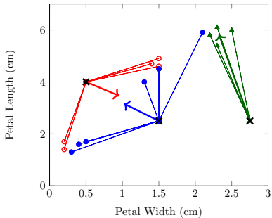
(b) membership assignment
