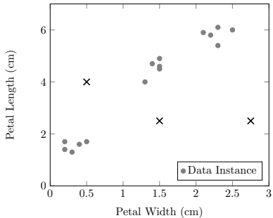
(a) initial (random) centroids
