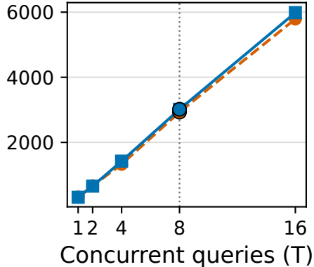
YFCC-10M
