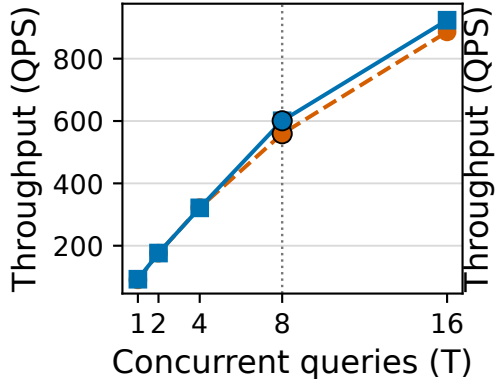
T2I-10M
