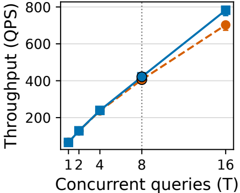
LAION-10M
