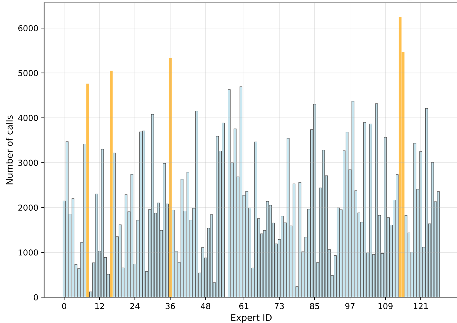
humaneval_thinking_off - Expert Usage Distribution - layer_1
