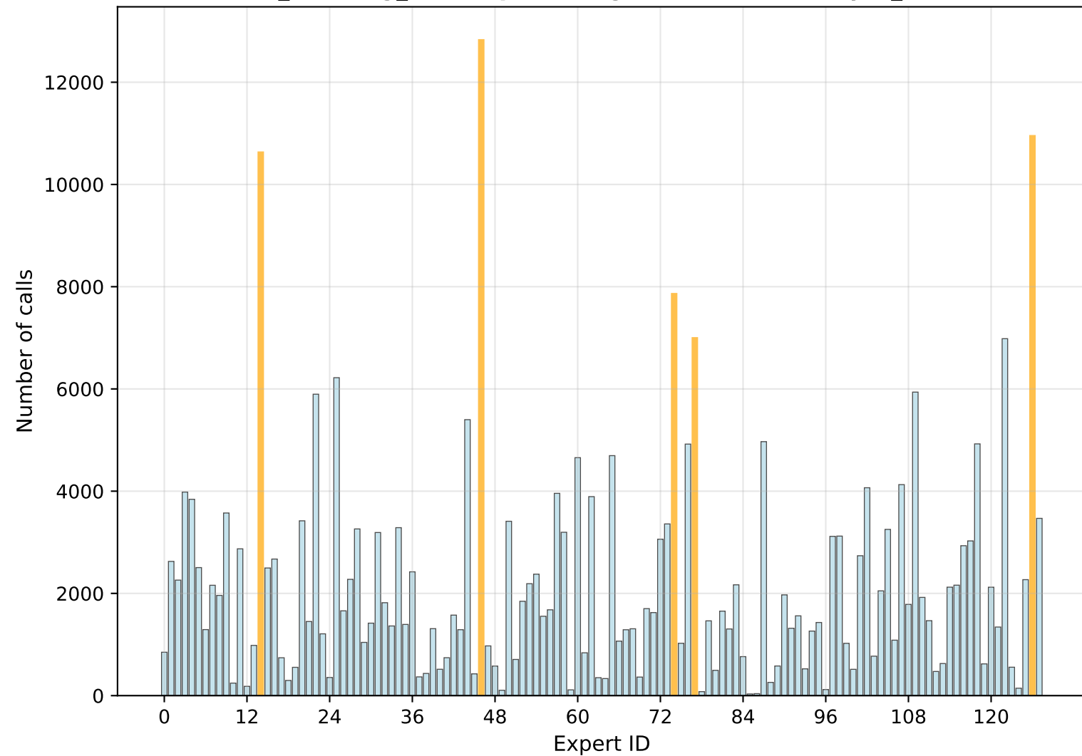
humaneval_thinking_off - Expert Usage Distribution - layer_48 (index -1)
