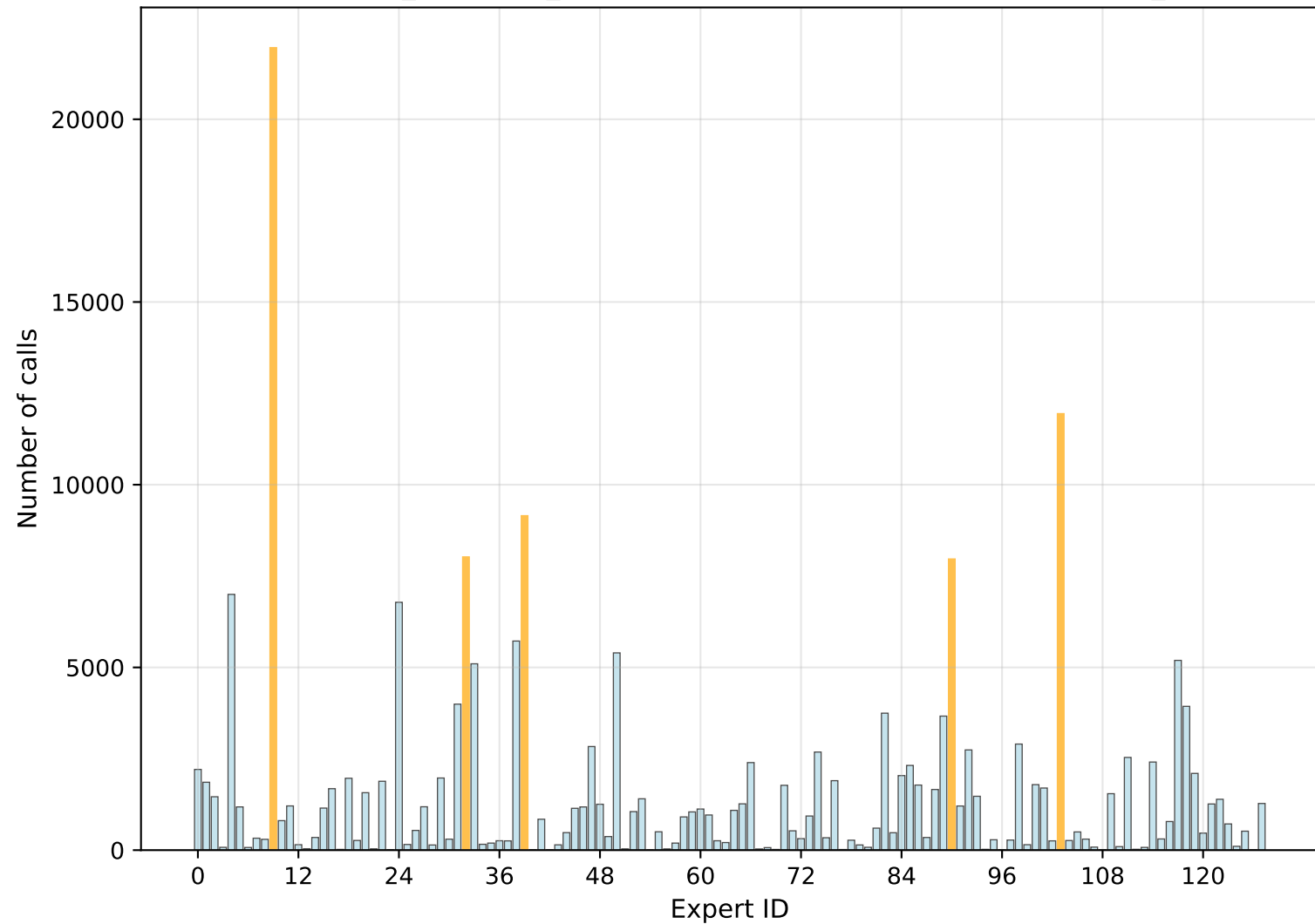
wikitext_thinking_off - Expert Usage Distribution - layer_1
