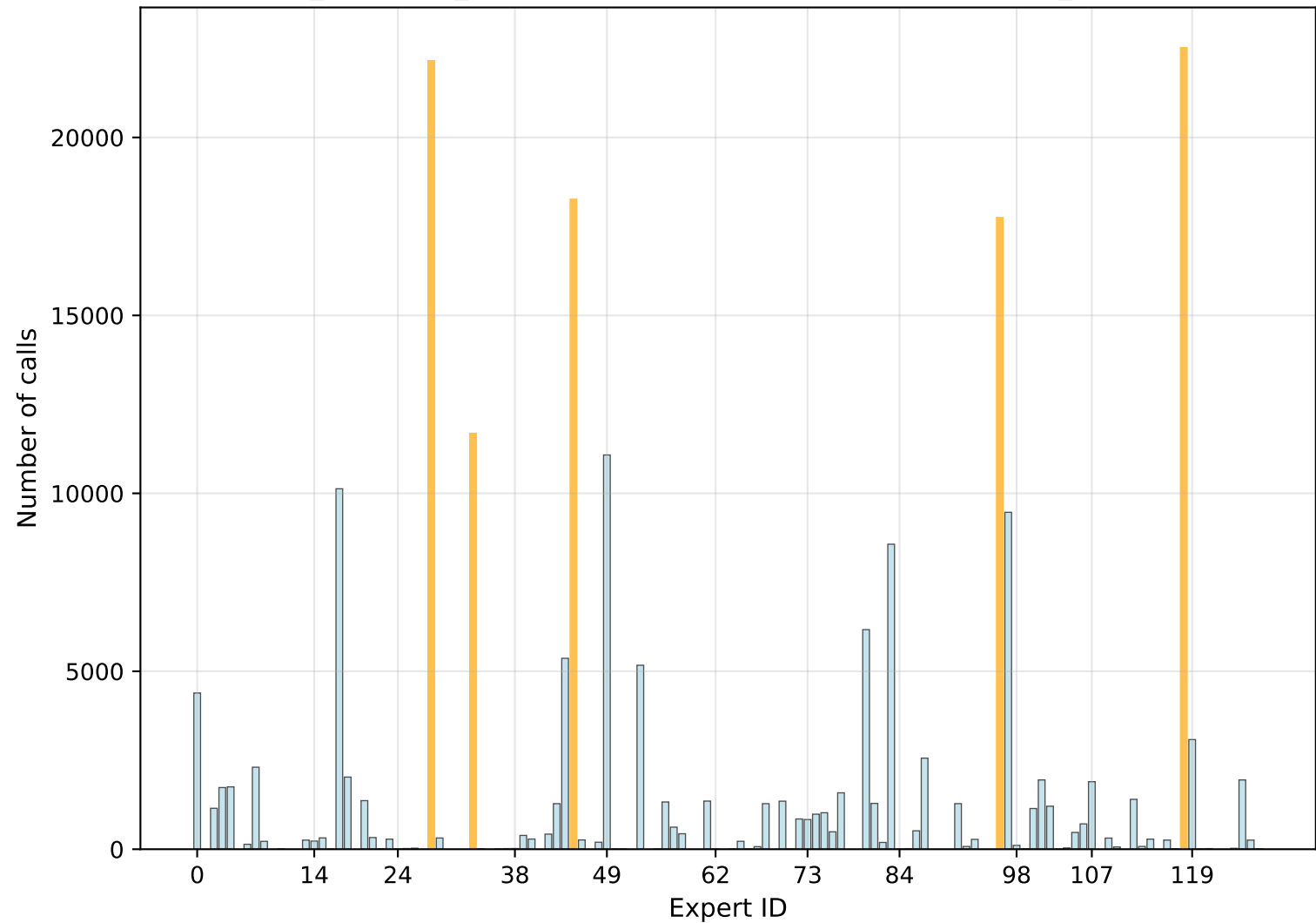
wikitext_thinking_off - Expert Usage Distribution - layer_48 (index -1)
