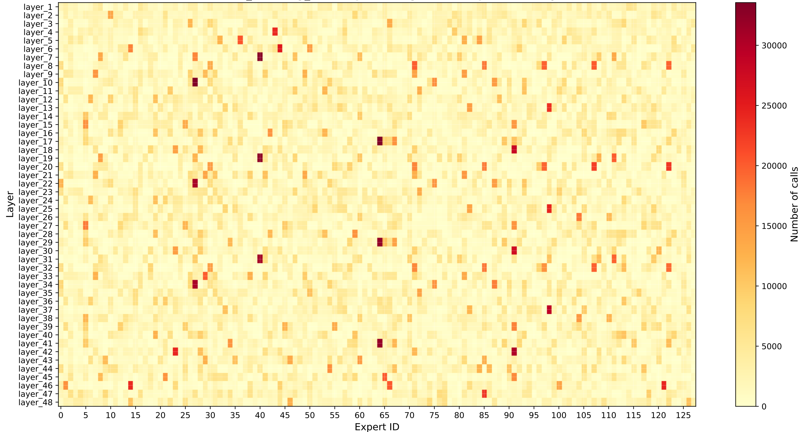
humaneval_thinking_off - Expert Usage Heatmap Across Layers
