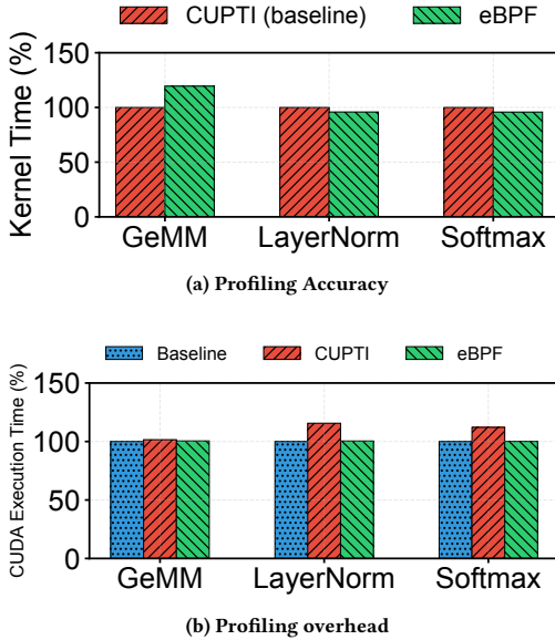
Figure 2: Profiling Results
