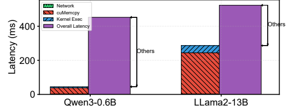
Figure 6: Performance Breakdown
