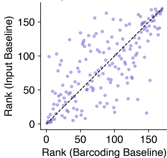
Spleen R_p = 0.77 \mid R_s = 0.70
