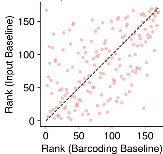
Meninges R_p = 0.53 \mid R_s = 0.53
