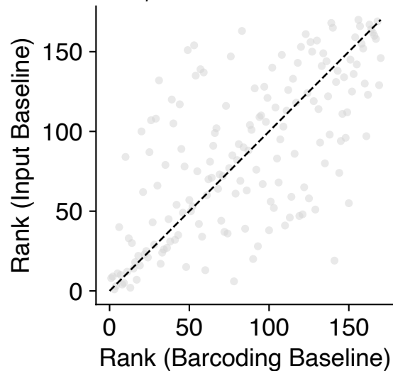
In Vitro R_p = 0.70 \mid R_s = 0.67
