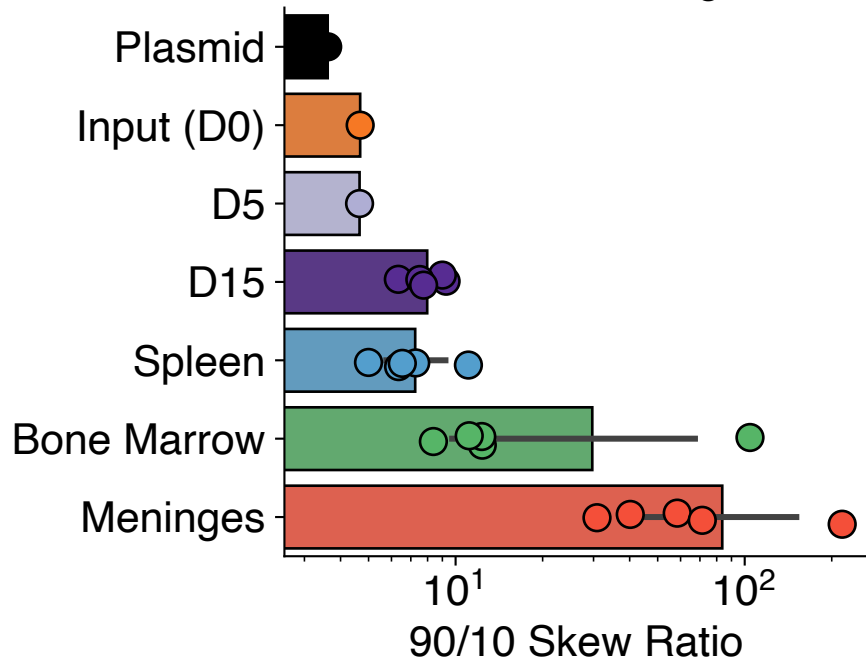
ABE Barcoding
