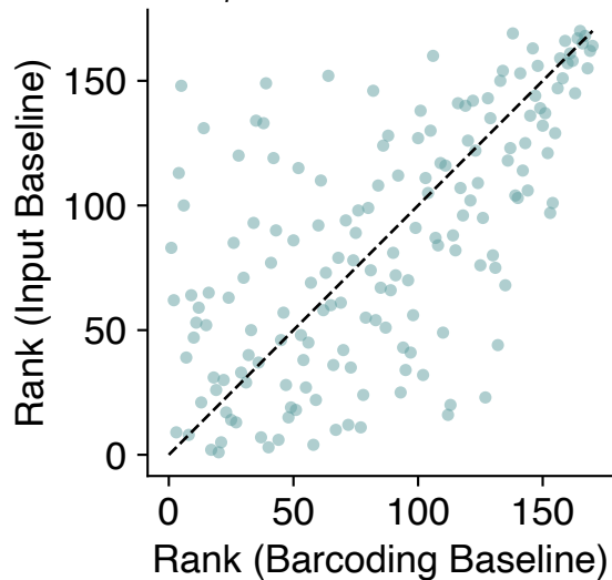
Bone Marrow R_p = 0.62 \mid R_s = 0.63
