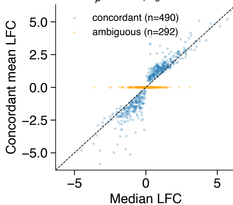
r_p=0.933 , r_s=0.947
