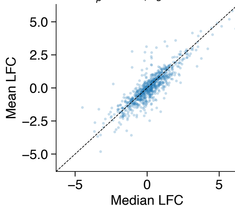
r_p=0.933 , r_s=0.947
