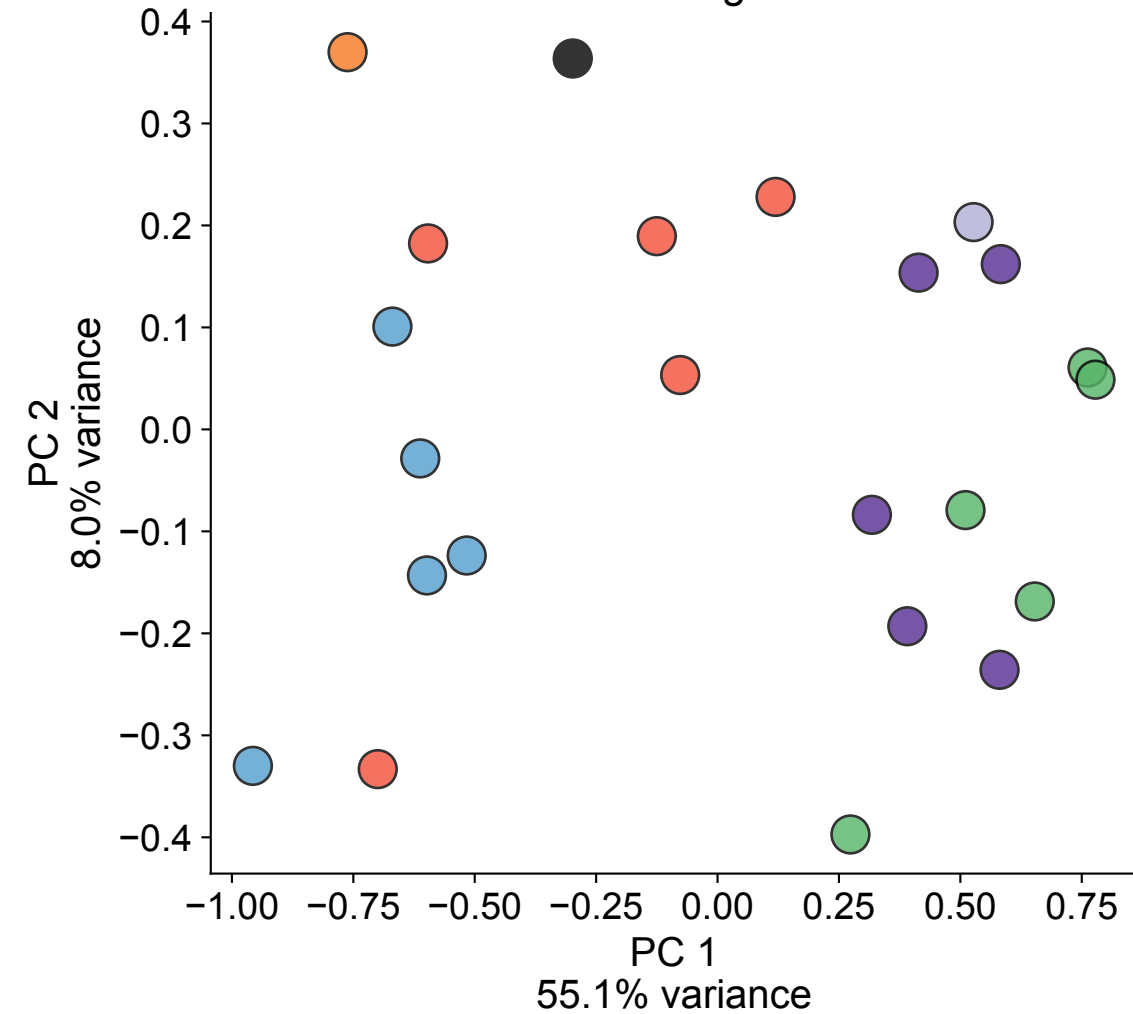
PCA on Correlation of BC Counts ABE barcoding screen
