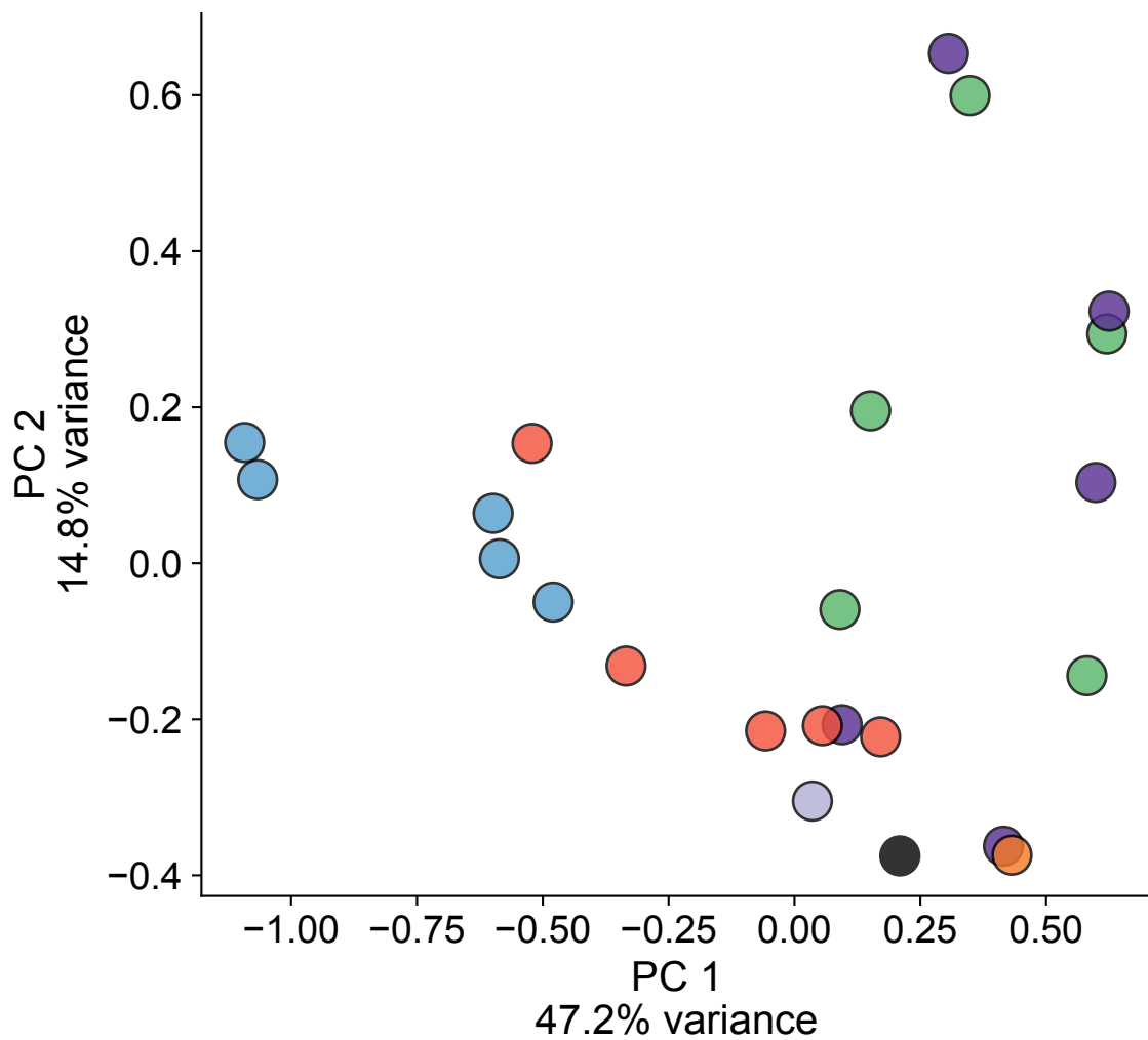
PCA on Correlation of BC Counts ABE EPO screen
